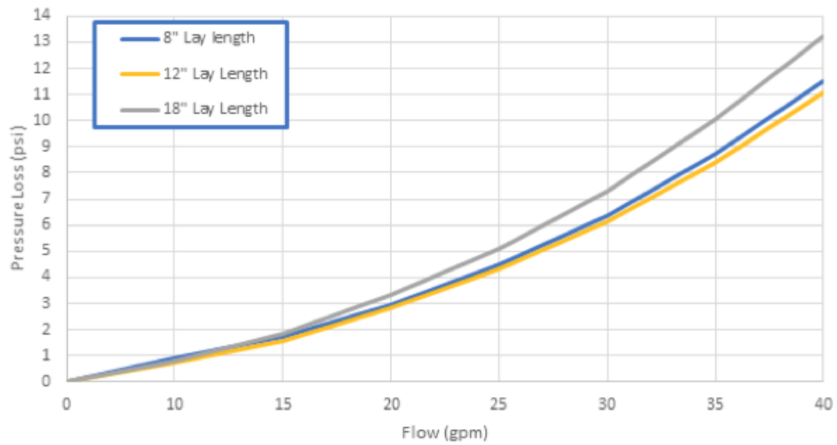
1" Swing Joint Pressure Loss
