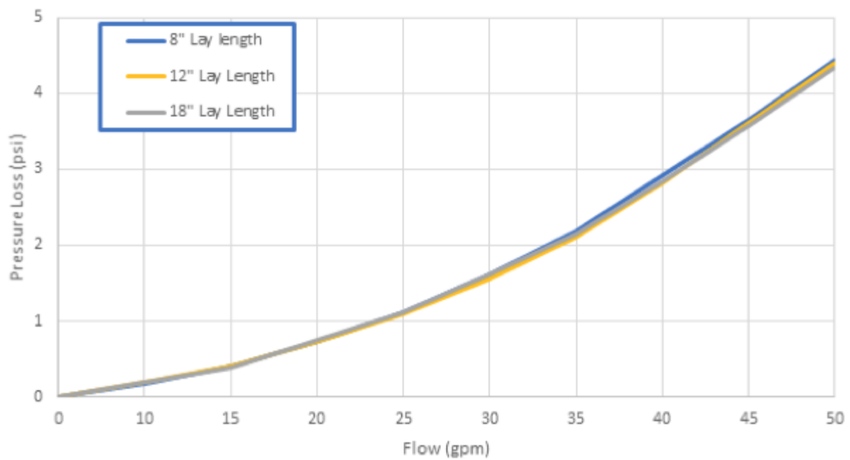
1.25" Swing Joint Pressure Loss (0-50 gpm)
