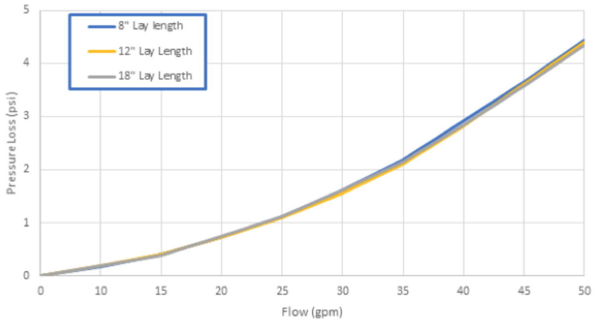
1.25" Swing Joint Pressure Loss (0-50 gpm)
